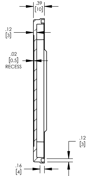
SECTION D-D COVER
