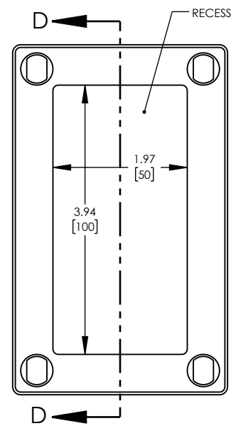
COVER - TOP VIEW
