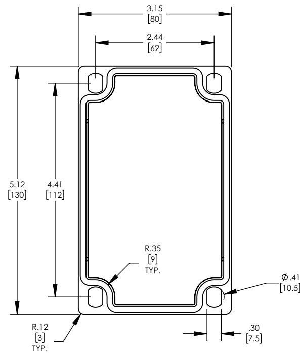
COVER - BACK VIEW
