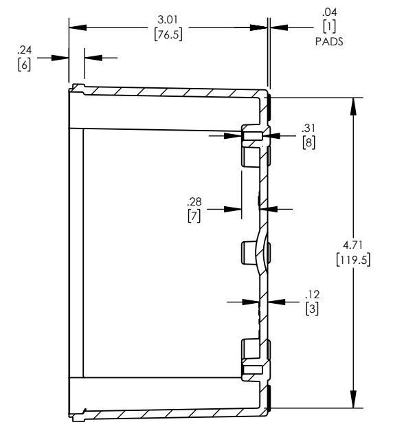
SECTION E-E
